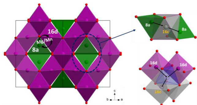
Figure 1. \text{MgCrMnO}_4 crystal structure (space group Fd\bar{3}m ) with 16d octahedra shown in purple, vacant 16c octahedra shown in gray, and 8a tetrahedra shown in green. The possible diffusion pathways of \text{Mg}^{2+} (8a), \text{Mg}^{2+} (16d), and \text{Mn}^{2+} (8a) are shown on the right, in which right edges of the 16c octahedron are colored in purple indicating the edge sharing with 16d octahedra.
