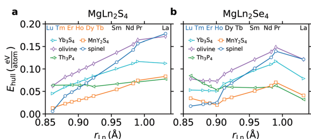
Fig. 5 Stability with respect to competing phases, E_{\text{hull}} for each sulphide (a) and selenide (b) in a variety of crystal structures common to AB 2 X 4 -type compounds. The colour of each element at the top of both panels correspond with the experimentally observed crystal structure for that composition. 27,30 MgTm 2 S 4 is coloured for both spinel and MnY 2 S 4 because both crystal structures have been reported. Elements coloured black indicate no experimentally known crystal structure.
