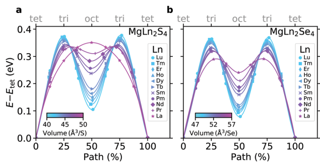
Fig. 3 Energy profiles for vacancy-mediated Mg^{2+} migration in sulphides (a) and selenides (b). Energy is shown relative to the tetrahedral Mg state ( E - E_{tet} ). The colourbar provides the volume per anion of the pristine structure.
